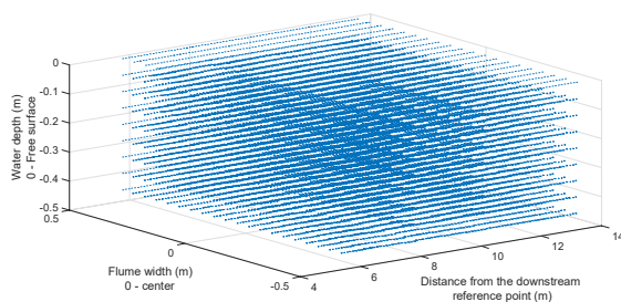
Figure 5: Quiver of velocities according to the flume coordinate system.
