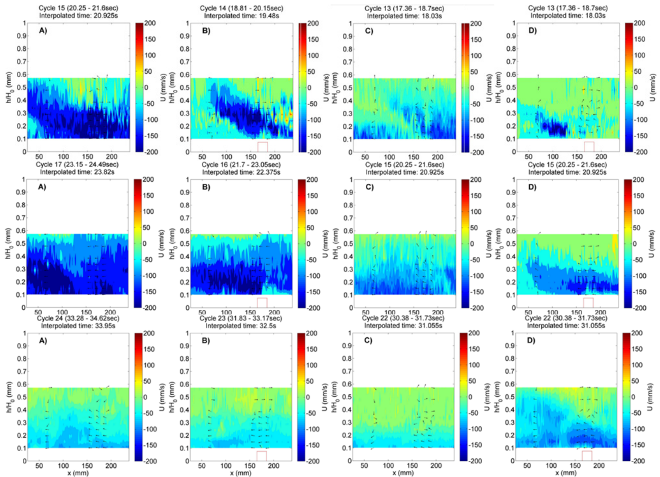
Figure 2: Horizontal velocity contour plots with directional vectors of setup A, B, C and D; (top) first cycle; (middle) third cycle; (bottom) tenth cycle. The x-axis represents distance from horizontal transducer tips.
