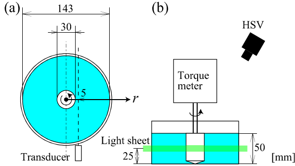
Figure 1: (a) The top view and (b) the side view of the experimental apparatus
