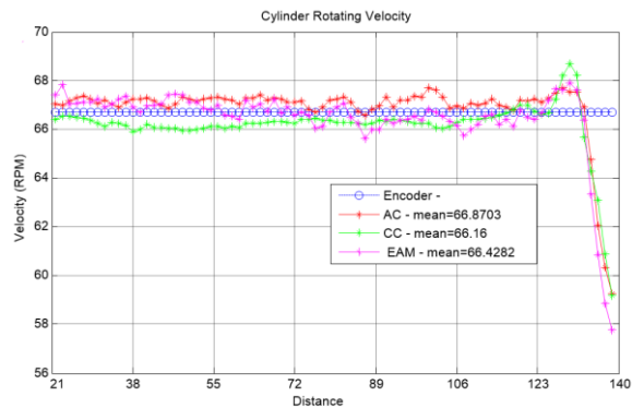
Figure 4: Velocity profile for 65RPM
