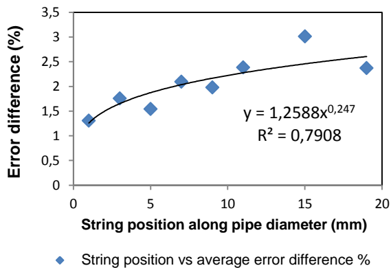
Figure 6: Average velocity error vs. depth positions (absolute error).
