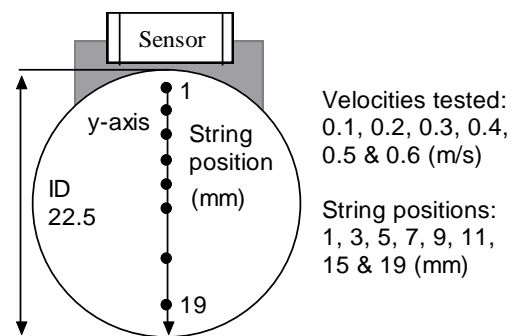
Figure 2: String positions and velocity range tested.
