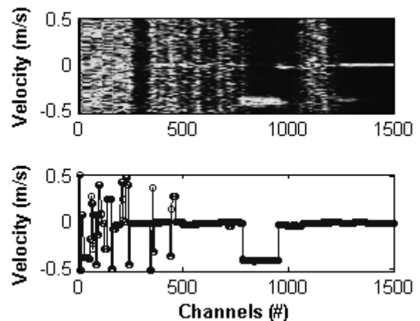
Figure 4: Doppler spectra and corresponding velocity measurement for 11 mm depth and 0.4 m/s string speed.
