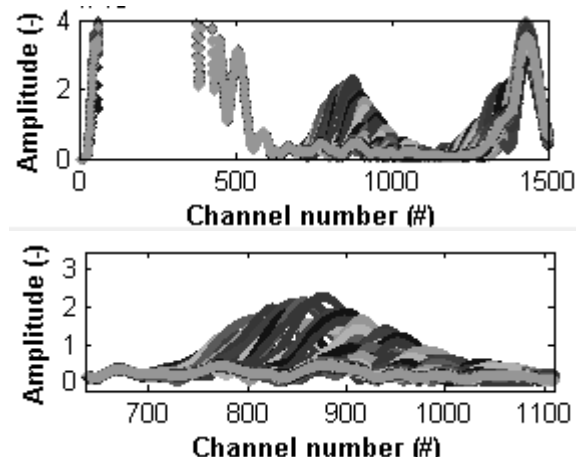
Figure 3: Magnitude of complex signal showing sampling volume axial extension. The bottom panel is a zoom between gates 600 and 1100. Each line is a received echo from an emitted pulse.
