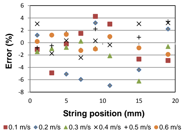
Figure 5: Deviation of measured velocity from string velocity vs. depth positions.
