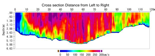
Figure 4 cross section velocity distribution
