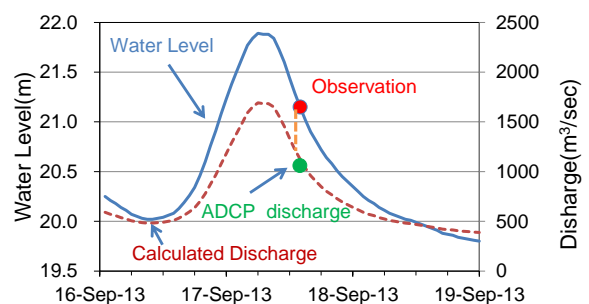
Figure 2: Hydrograph of the flood in Ishikari River
