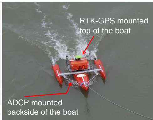
Figure 3: ADCP Boat system
