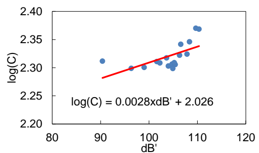
Figure 6: Relation Turbidity to Backscatter
