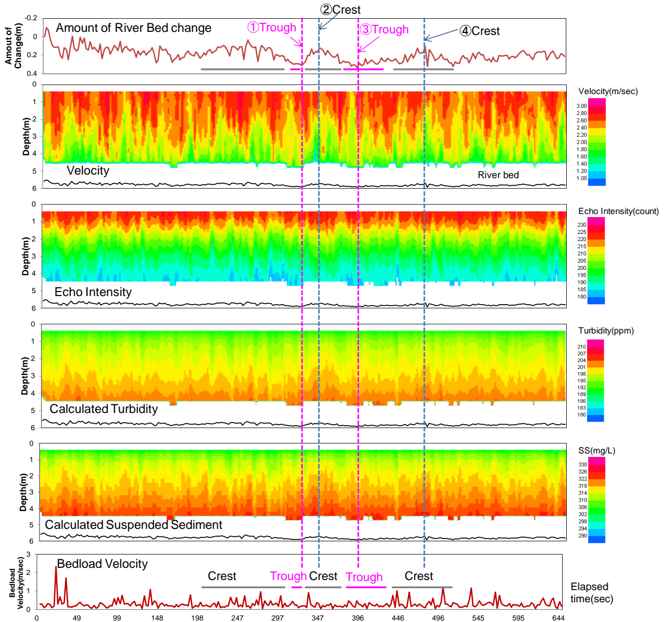
Figure 8: ADCP time series observation during flood
