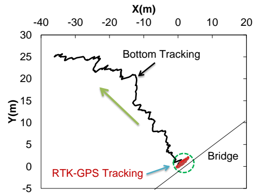
Figure 5: Bed moving observation
