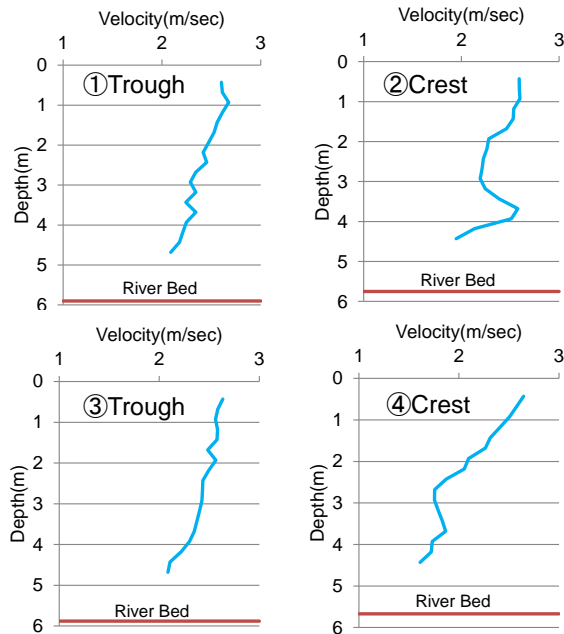
Figure 9: Velocity Vertical profile
