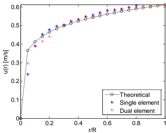
Figure 5: Comparison of velocity profile measured for J_L=0.5 m/s.
