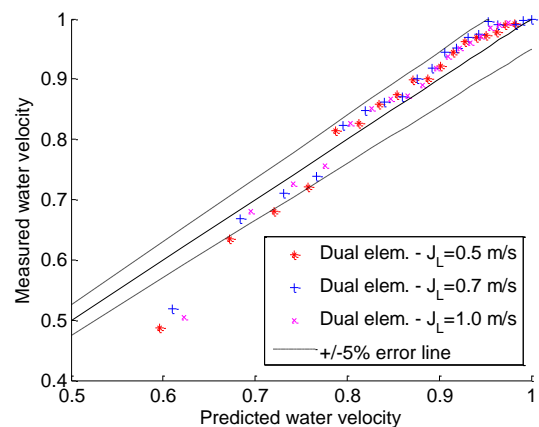
Figure 8: Comparison of predicted to measured water velocity for dual element transducer (5 MHz).
