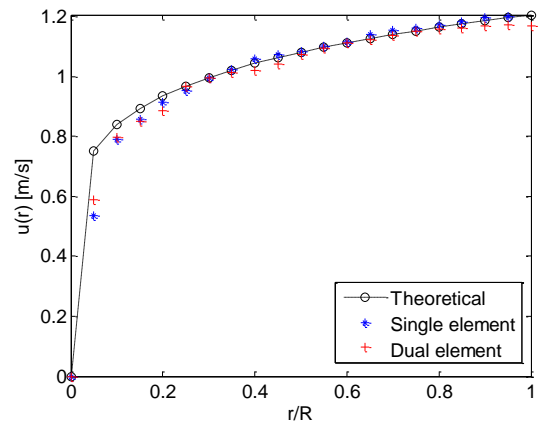
Figure 7: Comparison of velocity profile measured for J_L=1.0 m/s.
